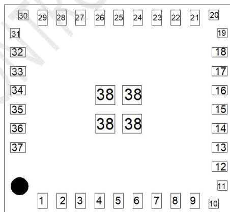
Figure 2.2: HJ-380IMH Pins distribution diagram(front view)
